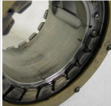
Journal/Thrust Bearings
